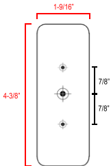
Outside Handle
